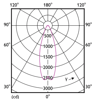
Light Distribution Diagram - MAS LEDEExpertColor 20-100W 930 AR111 24D
