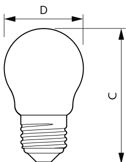
Candle P45 EU 3.5-40W 475lm WG E27 CL
