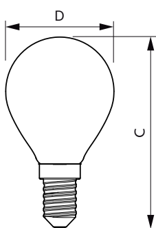
Candle P45 EU 2-25W 270lm WG E14 CL
