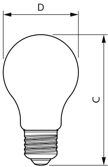
A60 230V 6-40W 470lm 2700K E27 D CL
